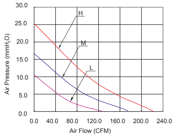
Performance Curves
